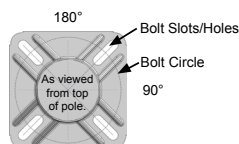
Anchor Base Detail
