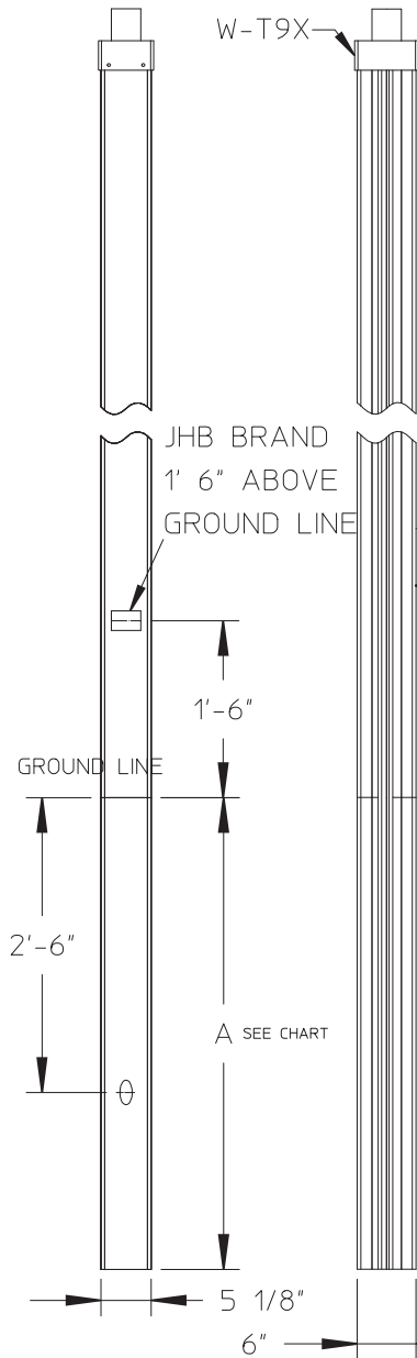
P STYLE POLE BURY DEPTH CHART
