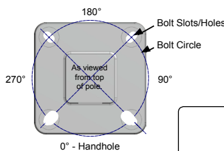
Anchor Base Detail
