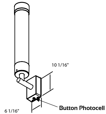
IW Wall Mount
