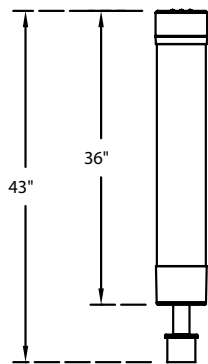
SF Slip Fit Mount
