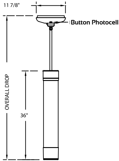
SH Stem Hung Mount
