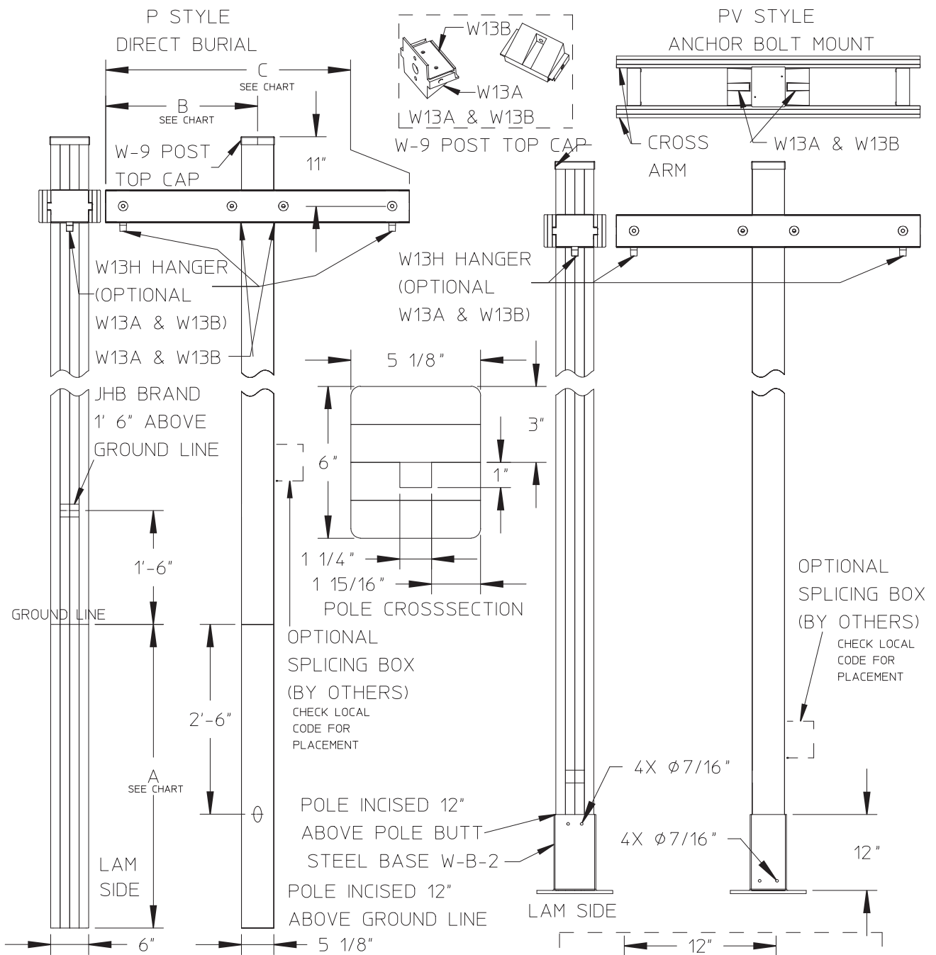
TWO WAY CROSS ARM CHART
